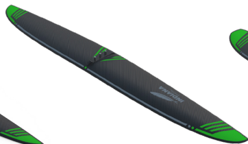
HP Front Wing Manta XL Proj. Area: 2047 cm 2 Span: 1396 mm Aspect Ratio: 9.5 Art. 3549SQ
