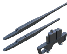
LIO-TEC Fuselage 715 Heavy Duty IN-AX Art. 8071SQ Fuselage 610 Heavy Duty IN-AX Art. 8072SQ Fuselage Adaptor IN-AX Art. 8073SQ
