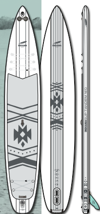
16'0 Touring Tandem Inflatable 16'0 x 34 x 6 | 485 L | 17.5 kg Art. 1006SQ
